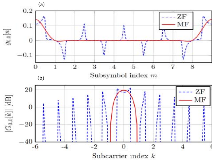
Fig. 4: Frequency and time characteristics of ZF and mfilters: a) Time impulse response and b) Frequency response
