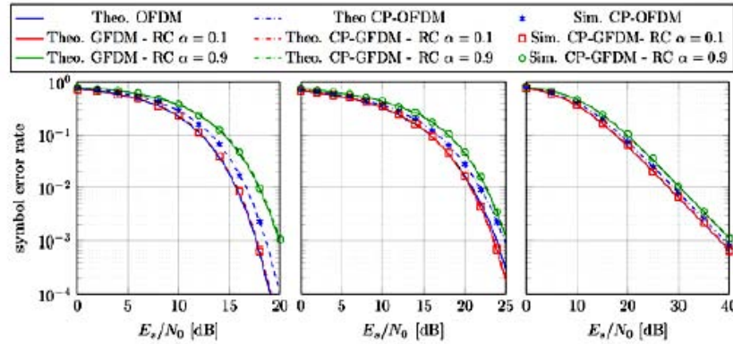
Fig. 5: Simulate the performance of GFDMM-SER under different channel models: a) AWGN channel; b) FSC channel; c) TVC channel
