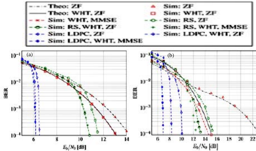
Fig. 7: Simulation of BER performance for combined scheme WHT-GFDM: a) Ch. A; b) Ch. B
