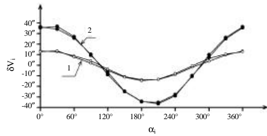
Fig. 2: Curves for deviations along the vertical circle; 1: regular force moment; 2: increased force moment
