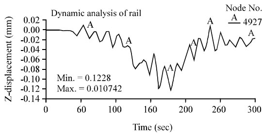
Fig. 4: Deformation of reinforced ballasted track for a train speed of 350 km h -1
