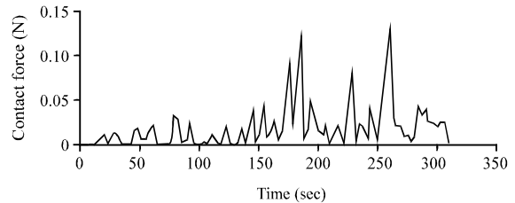
Fig. 9: Contact force
