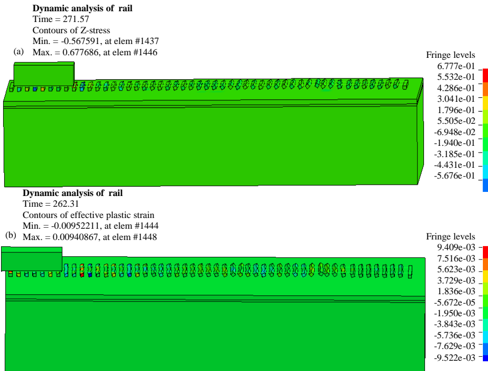
Fig. 7: a) stress in a non-reinforced ballasted railway for a train speed of 350 km h -1 and b) plastic strain in a non-reinforced ballasted railway for a train speed of 350 km h -1
