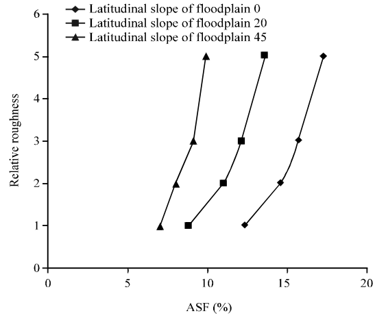
Fig. 10: Size of the roughness at the main channel 0.01 m and relative width 2.5 m
