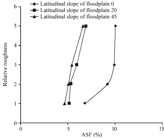
Fig. 2: Size of the roughness at the main channel 0.000131 m and relative width 1.25 m
