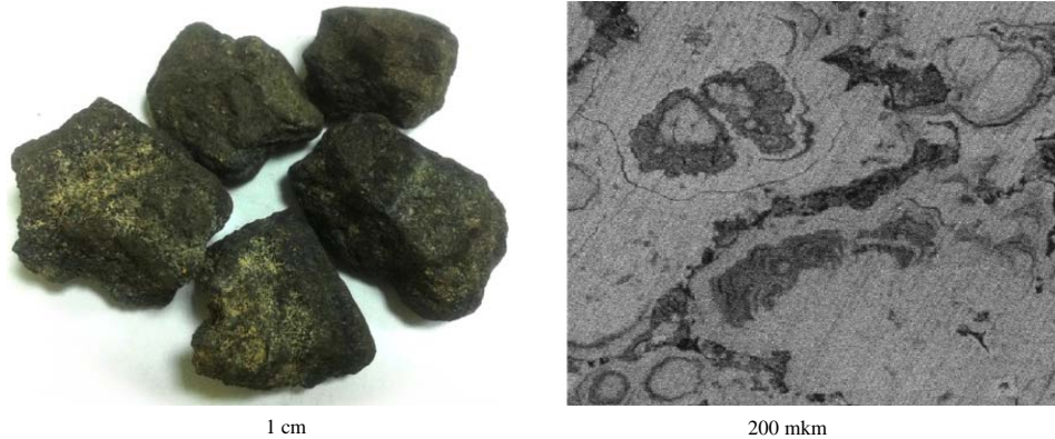
Fig. 2: Ferro manganese concretions of clarion-clipperton field
