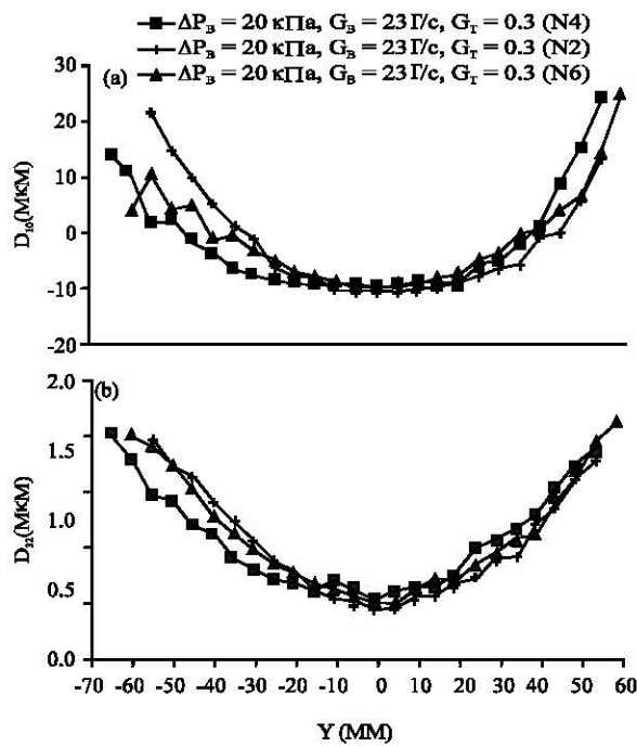
Fig. 6: Distribution medium D10 and medium Zauter D32 fuel particle diameter in the spray; MkM: TyT далее; MM: mkM; kPa: mm: kPa
