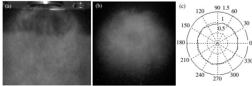
Fig. 5: Photos of the aerosol burner with fuel and pneumodispersion photograph of a cross section of the laser knife and circumferential fuel uneven
