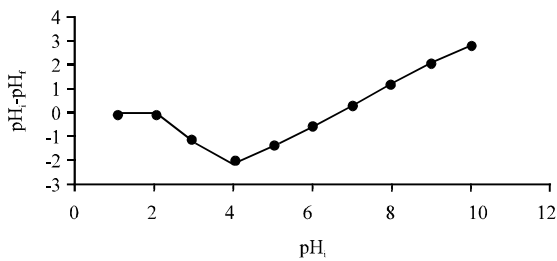
Fig. 5: The plot of \text{pH}_i - \text{pH}_f against \text{pH}_i . (Conditions: agitation speed: 150 rpm; biocarbon dose: 0.1 g; \text{pH} : 1-10; contact time: 24 h; room temperature: 25 \pm 2^\circ\text{C} ; volume of NaCl solution: 50 mL; particle size: \leq 150 \mu\text{m} )
