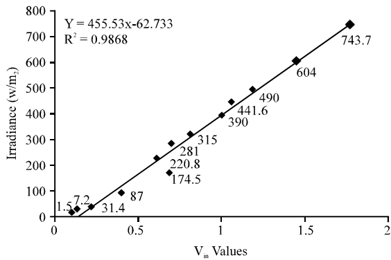
Fig.10: The linear of V_m = f (Irradiance) of the silicon sensor
