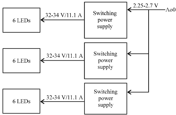
Fig. 6: The control of the artificial irradiance diagram
