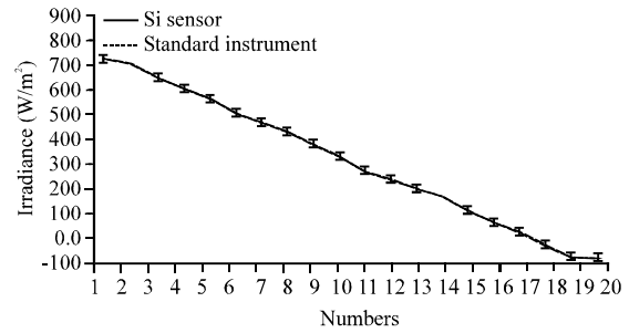
Fig. 14: The irradiance measured from silicon sensor, standard pyranometer
