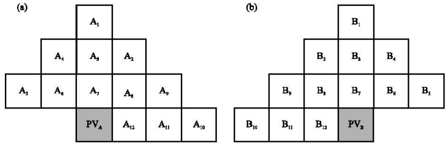
Fig. 1: Pixel value prediction using neighbor 12 pixel values: a) Odd-numbered line and b) Even-numbered line
