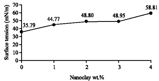
Fig. 4: Surface tension of modified AAM solution surface tension
