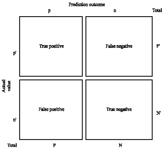
Fig. 5: Confusion matrix
