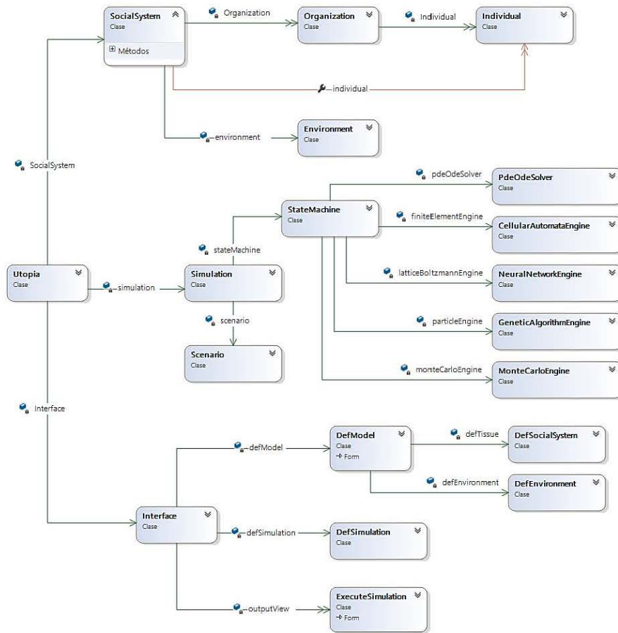
Fig. 1: An UML (Unified Modeling Language) class diagram
