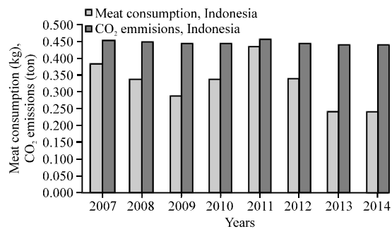
Fig. 3: Meat consumption and CO 2 emissions in Indonesia
