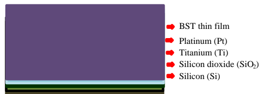
Fig. 2: 3D cross-section of thin films
