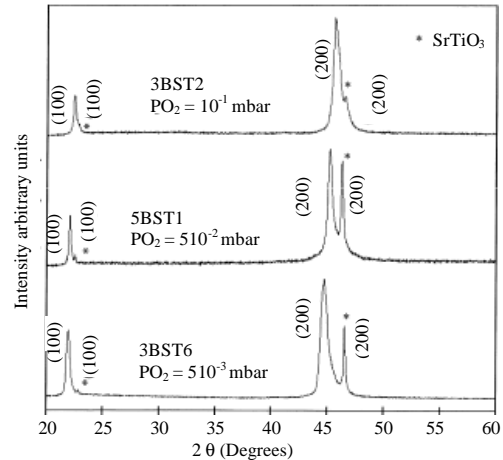
Fig. 1: XRD pattern of pulse laser deposition (Goux et al. , 2001)
