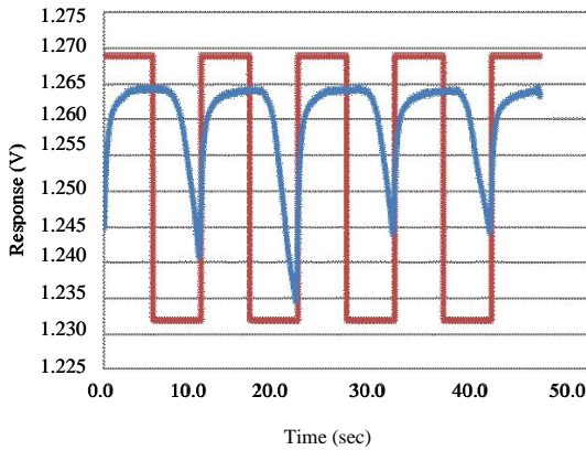
Fig. 4: Response time measurement via. testing jig
