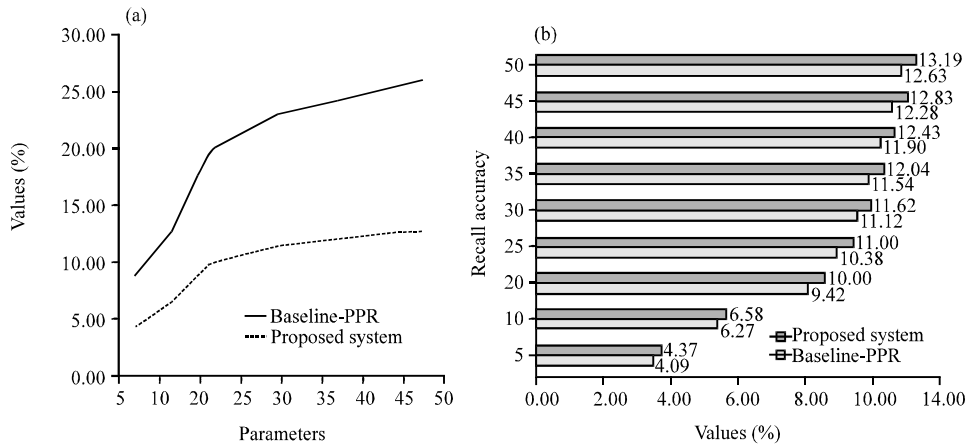
Fig. 4: Comparison of systems using F-measure
