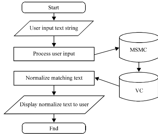
Fig. 3: Normalization process
