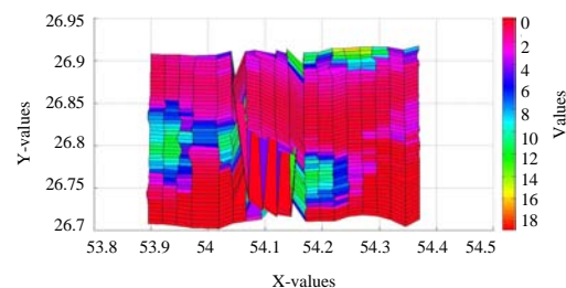
Fig. 1: Complete bouguer anomaly with density (2.6) g/cm 3
