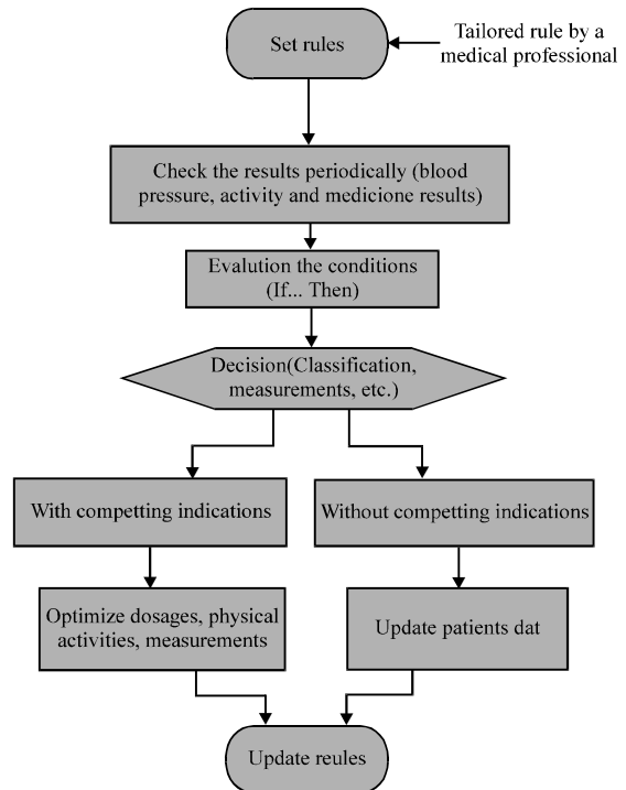
Fig. 3: Rule-based reasoning
