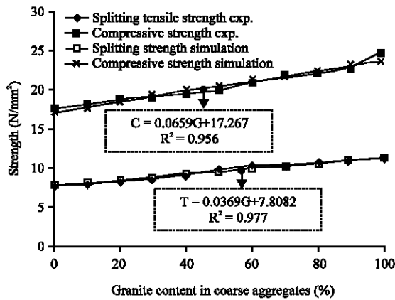
Fig. 7: Plots of splitting tensile and compressive strengths against granite content in coarse aggregates for 1:2:4 concrete mix
