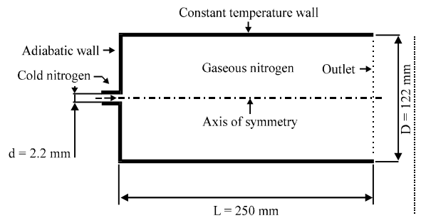
Fig. 1: Chamber geometry
