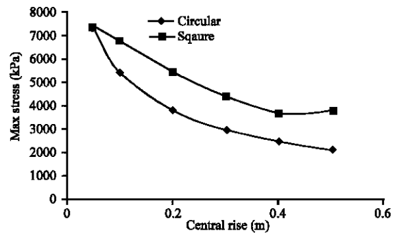
Fig. 9: Effect of the base shape on the maximum Von Mises stress of 0.10 m slab thickness
