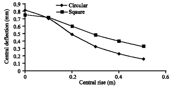
Fig. 8: Effect of the base shape on the central deflection of 0.20 m thick slab
