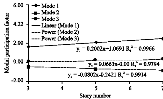
Fig. 12: Story number vs. modal participation factor
