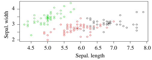
Fig. 1: K-means clustering
