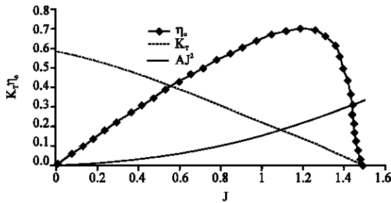
Fig. 1: Intersections examples
