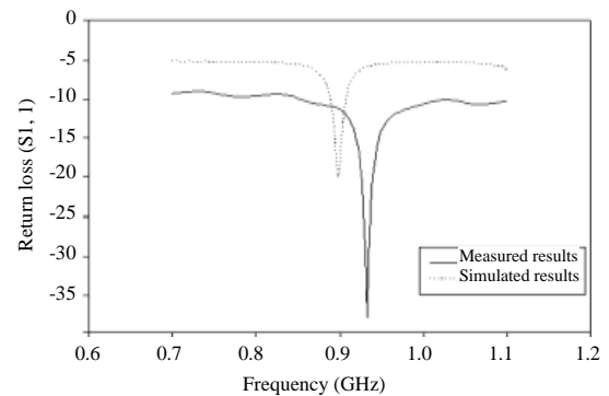
Fig. 6: Comparison between simulated and measured results of return loss curve using Sigma Plot 10.0
