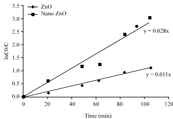
Fig. 7: Kinetics analysis for carmine dye (dye initial concentration 40 ppm), (1g ZnO) and 0.75 g nano ZnO
