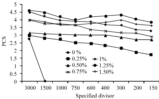
Fig. 15: The Post Crack Strength (PCSm) for all fibers percentages
