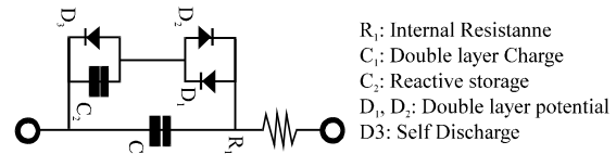
Fig. 3: Circuit model for simulation
