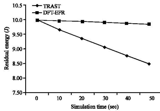
Fig. 6: Residual energy of TRAST and DTF-EER
