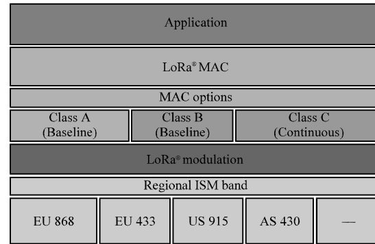
Fig. 1: LoRaWAN protocol, protocol specifications built on LoRa technology developed by LoRa alliance
