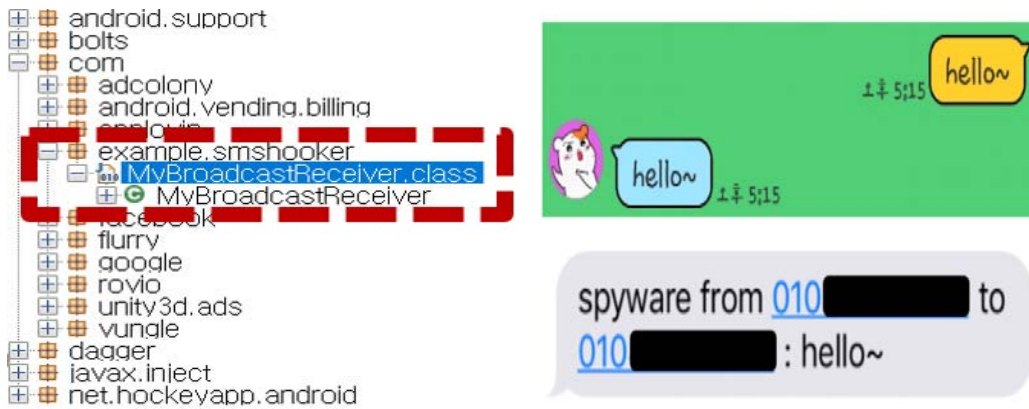
Fig. 3: Fake App. production result with malicious receiver code and its operation test
