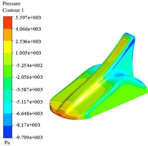
Fig. 7: Pressure result of H-type shark antenna model
