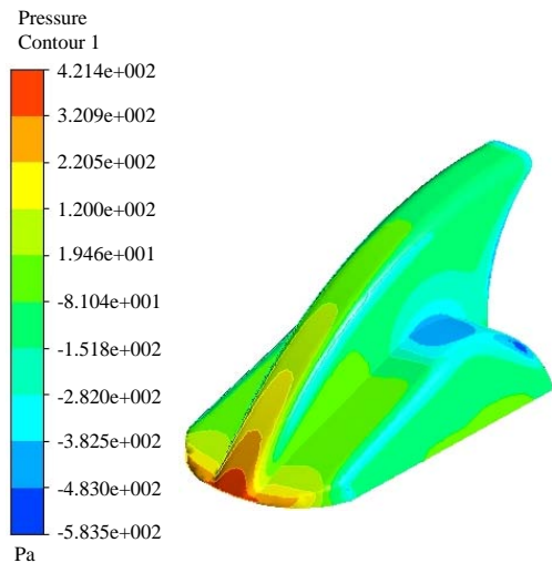
Fig. 8: Pressure result of K-type shark antenna model
