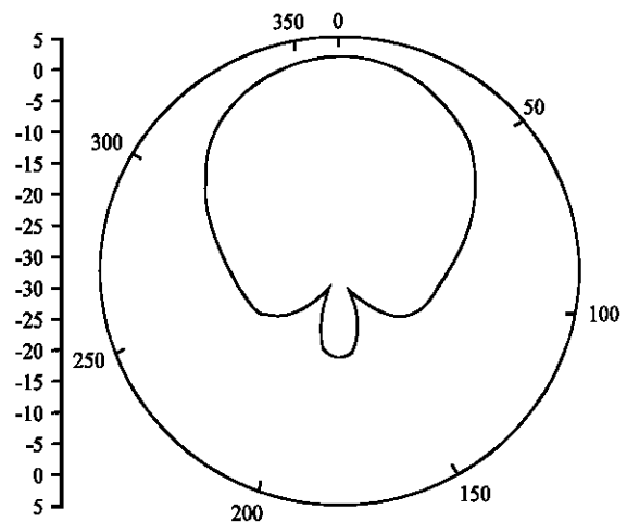
Fig. 5: Simulated radiation pattern at 8 GHz for antenna 2
