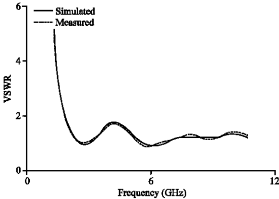
Fig. 6: Simulated and measured VSWR for antenna 2
