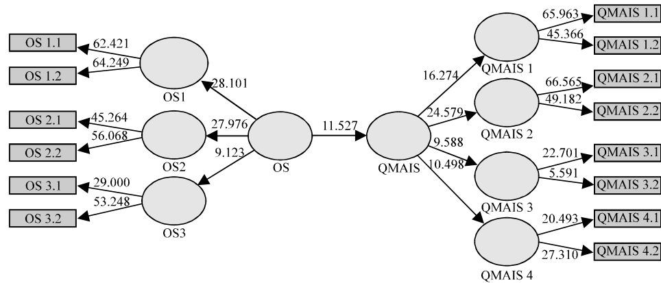
Fig. 2: Path diagram (Bootstrapping)
