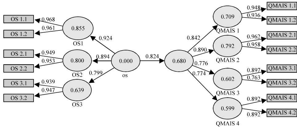
Fig. 1: Path diagram (PLS algorithm)
