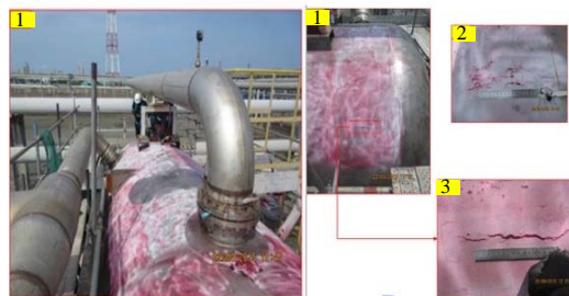
Fig. 6: Crack found at internal top tank same location as the external surface
