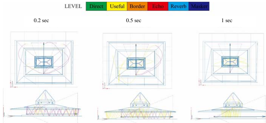
Fig. 4: Ray diagram for the complete model of Bangsal Srimanganti
