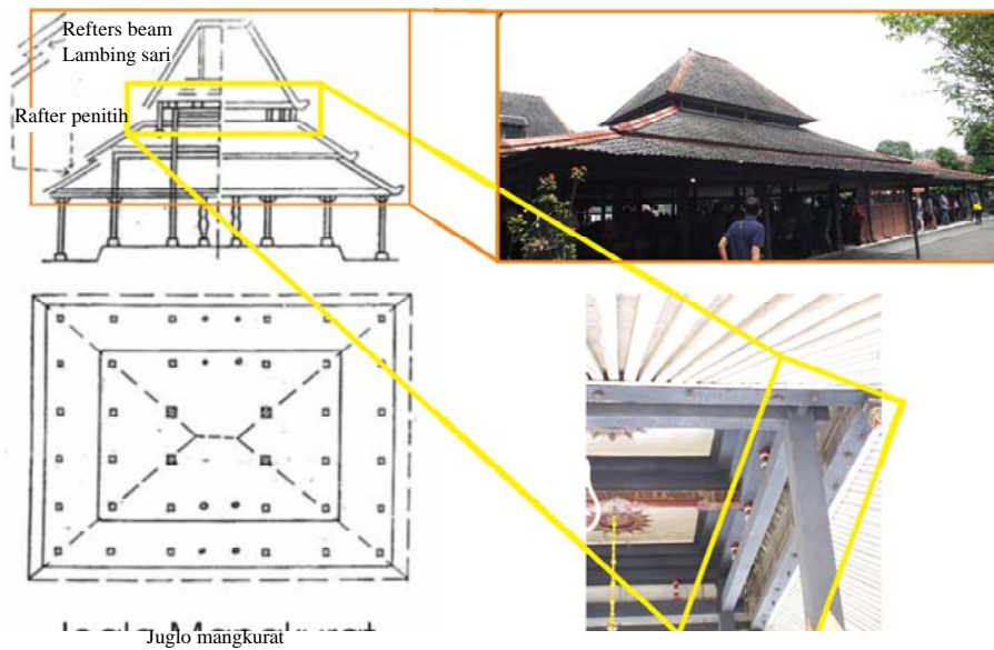
Fig. 3: Bangsal Srimanganti as Joglo Mangkurat with the existence of cylinder column
