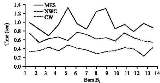
Fig. 10: Comparison of response times
