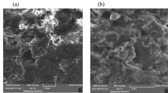
Fig. 6: SEM image of AC-BC mixture with 5% BGA
