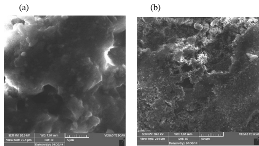
Fig. 7: SEM image of AC-BC mixture with 8% BGA
