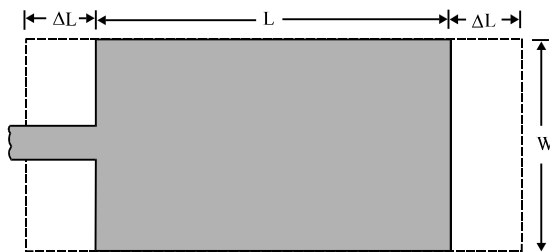
Fig. 2: Effective lengths of rectangular microstrip patch
