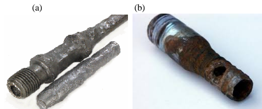
Fig. 4: Oxygen corrosion
