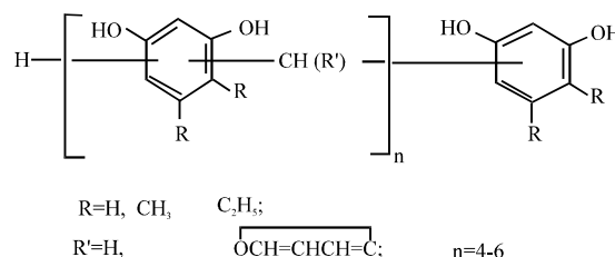
Fig. 3: Structural formula obtains resorcinol-aldehyde resin (Yurkevichyute et al. , 2016)
