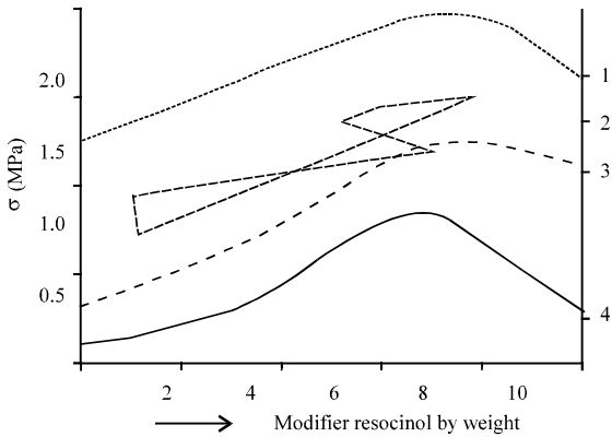
Fig. 4: Results of heat resistance of the mixture in terms of the residual strength of the samples, on the phenol-formaldehyde resin SFZH301 with different components of the modifier and different calcination temperatures: 1) At room temperature; 2) At 400, 3) 600 and 4 -800°C, respectively
