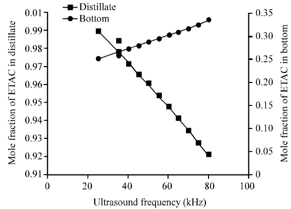
Fig. 6: Effect of ultrasound frequency on ETAC purity in the distillate of the UD column
