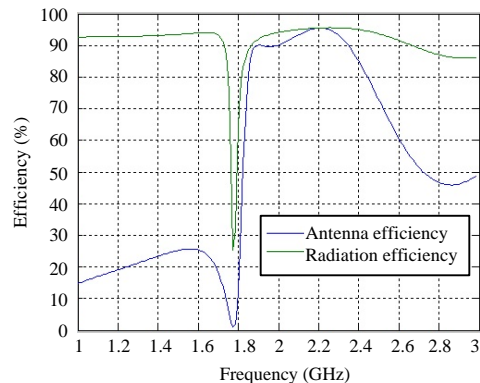
Fig. 6: Efficiency vs. frequency graph
