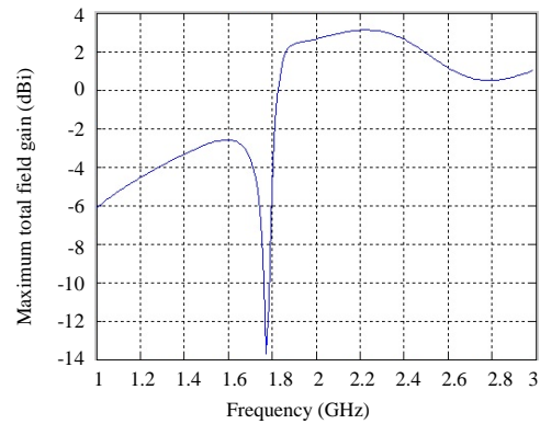
Fig. 5: Gain vs. frequency graph
