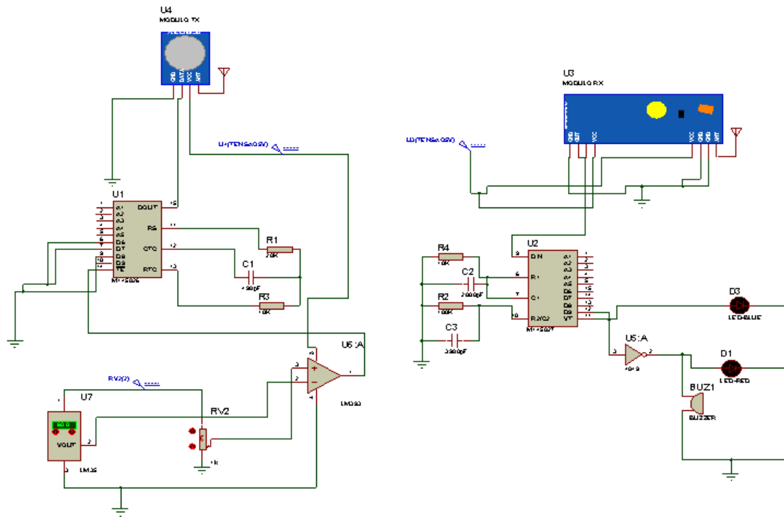
Fig. 5: Circuit diagram of RF based overhear alarm showing all components of the system
