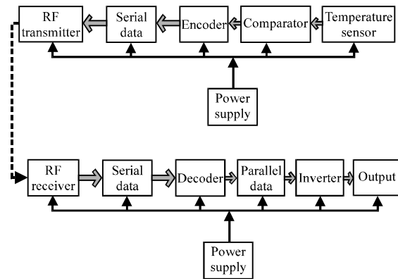
Fig. 4: Block diagram of RF based overhear alarm showing the major parts of the system
