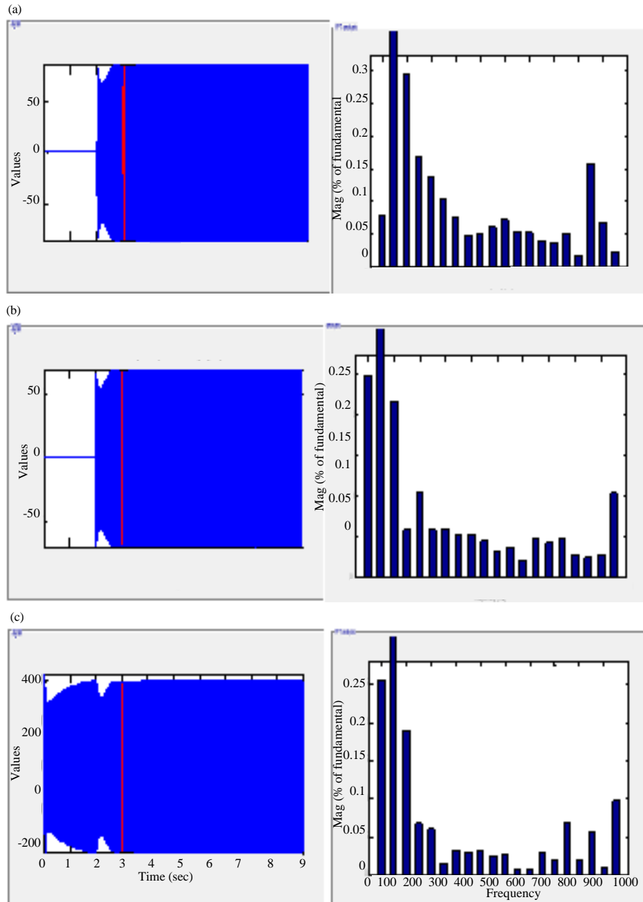
Fig. 15:IG THD analysis for; a) Load current; b) Phase voltage and c) Line to line load voltage; Selected signal: 500 cycles, FFT window (red): 1 cycles, Fundamental (50 Hz) = 84.73, THD = 0.45%; Fundamental (50 Hz) = 674.6, THD = 0.31% Fundamental (50 Hz) = 389.5, THD = 0.26%
