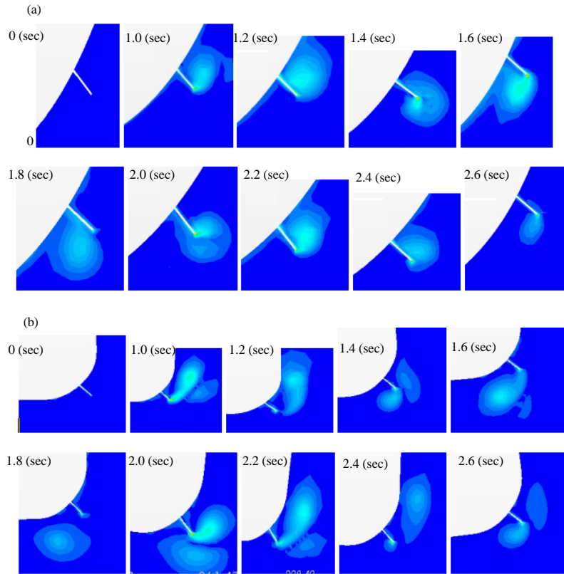
Fig. 2: a) Vorticity ( \text{sec}^{-1} ) evolution at section x/L = 0.729 , for a wave period of 5.2 sec and b) Vorticity ( \text{sec}^{-1} ) evolution at section x/L = 0.465 , for a wave period of 5.2 sec
