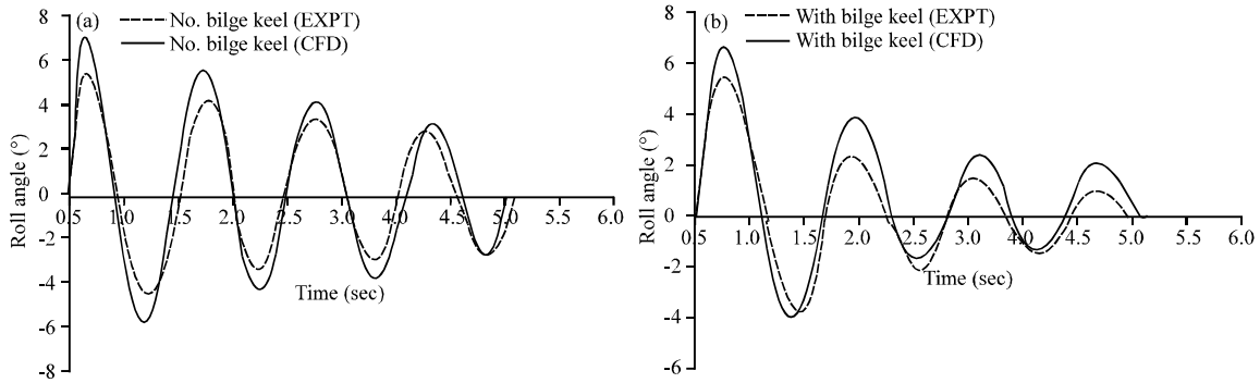
Fig. 4: Roll decay test time series with and without bilge keel: a) Roll response without bilge keel, period 1.12 sec and b) Roll response with bilge keel, period 1.20 sec
