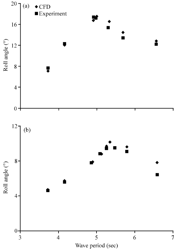
Fig. 6: Roll transfer function for prototype with and without bilge keel
