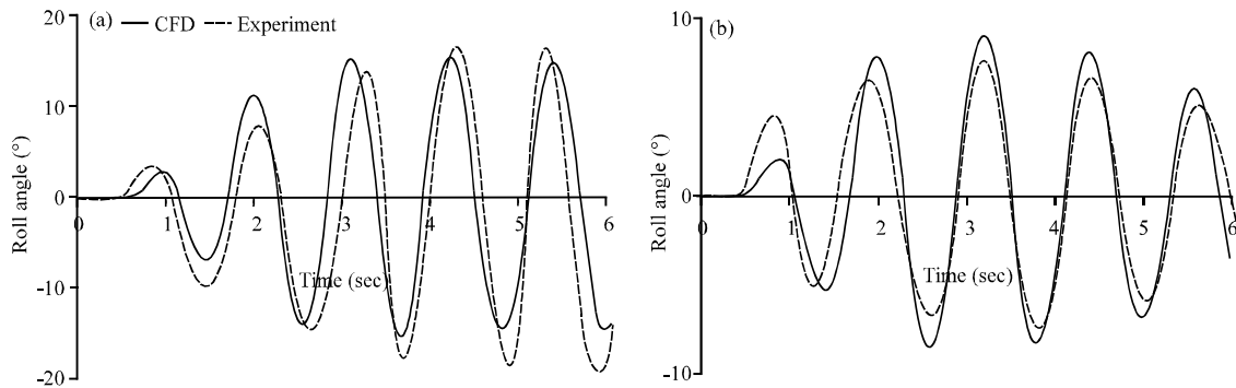
Fig. 5: Roll time series at respective resonance period with and without bilge keel (model scale): a) Without bilge keel and b) With bilge keel
