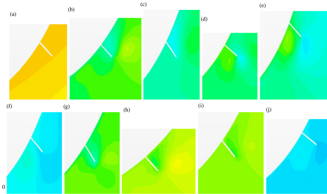
Fig. 3: Axial velocity (m/sec) contour at section x/L = 0.729 for a wave period of 5.2 sec: a) 0 (sec); b) 1.0 (sec); c) 1.2 (sec); d) 1.4 (sec); e) 1.6 (sec); f) 1.8 (sec); g) 2.0 (sec); h) 2.2 (sec); i) 2.4 (sec) and j) 2.6 (sec)
