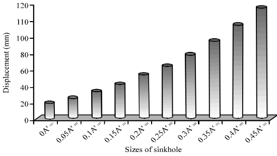
Fig. 6: Maximum displacements evolution with sizes of sinkhole
