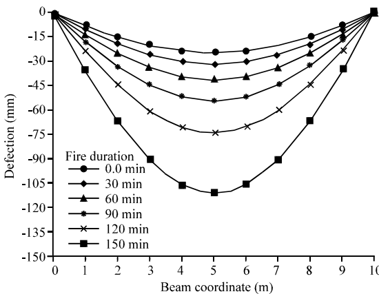
Fig. 8: Deflection curve of beam No. 2 at with different fire duratio
