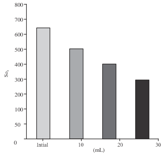
Fig. 26: Sulphate concentration value of sugar factory
