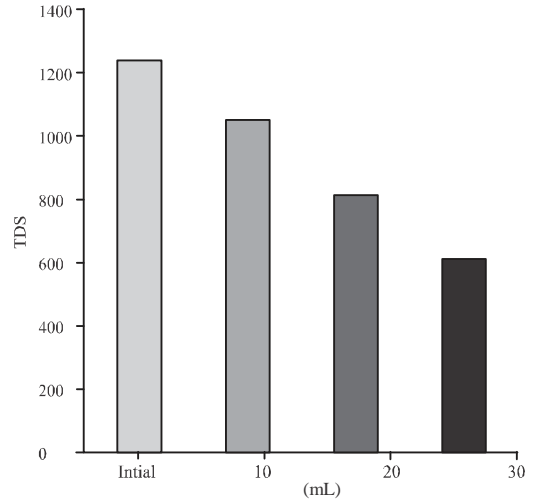
Fig. 14: Total dissolved solids value of sugar factory
